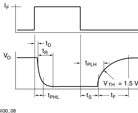
Fig. 8 - Switching Waveform
