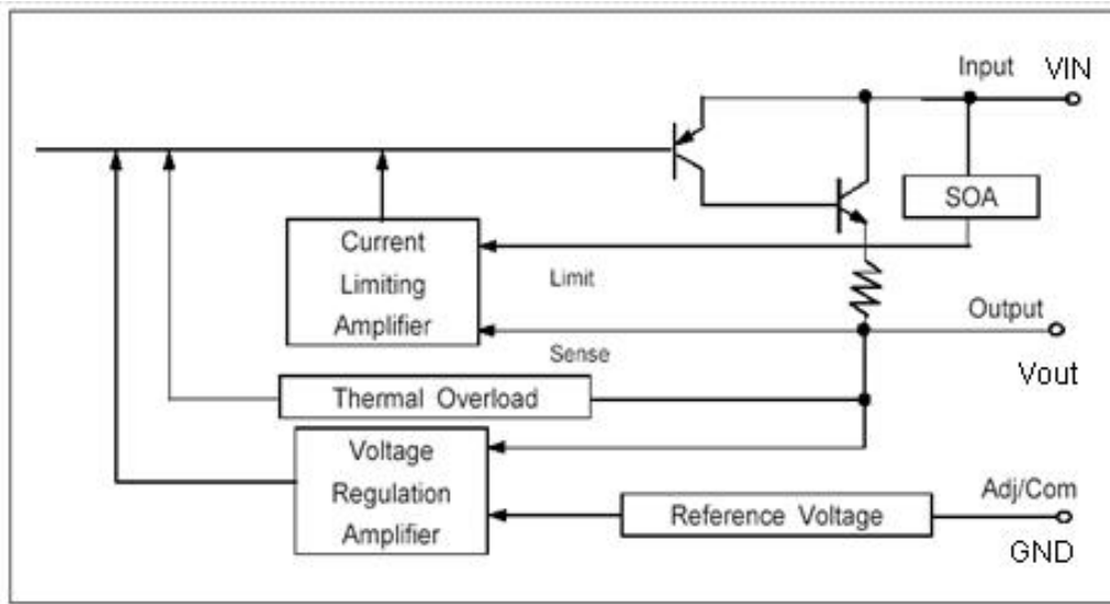
Block Diagram
