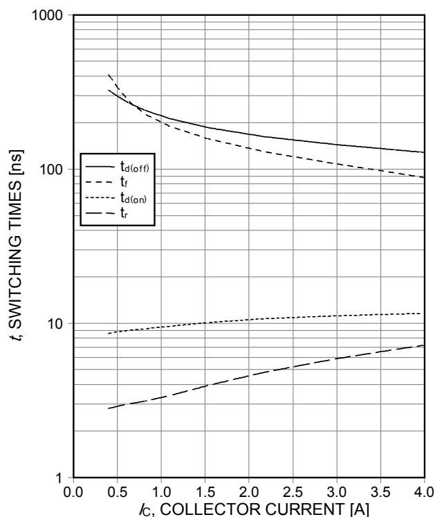
Figure 9. Typical switching times as a function of collector current (inductive load, T_{vj}=175^{\circ}\text{C} , V_{CE}=400\text{V} , V_{GE}=15/0\text{V} , r_G=43\Omega , Dynamic test circuit in Figure E)
