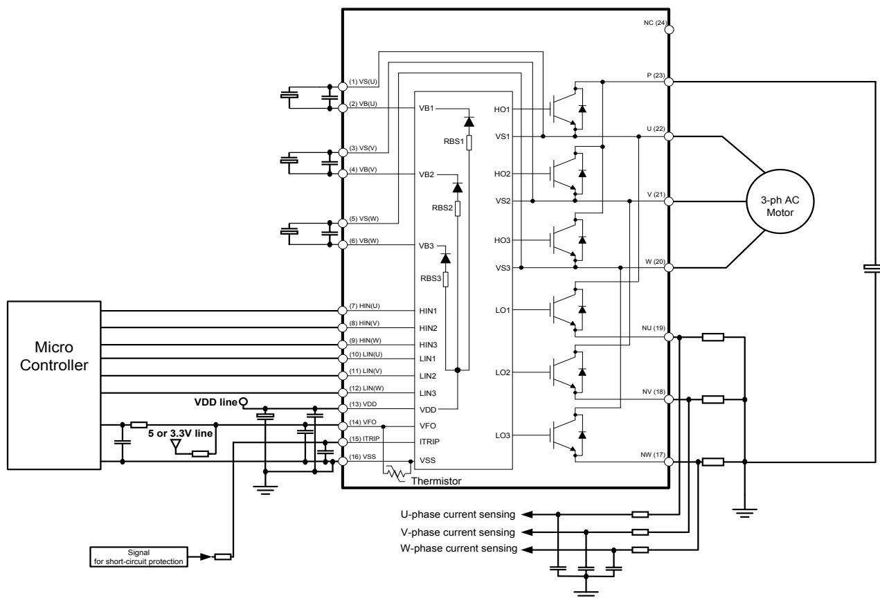
Figure 9: Application circuit
