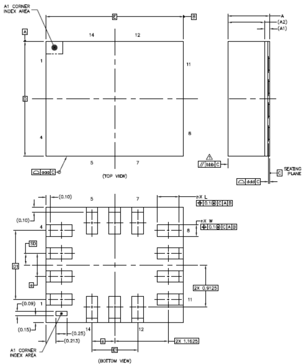
Figure 17. Package Dimensions
