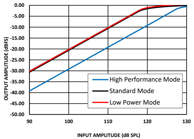
Figure 7. Linearity
