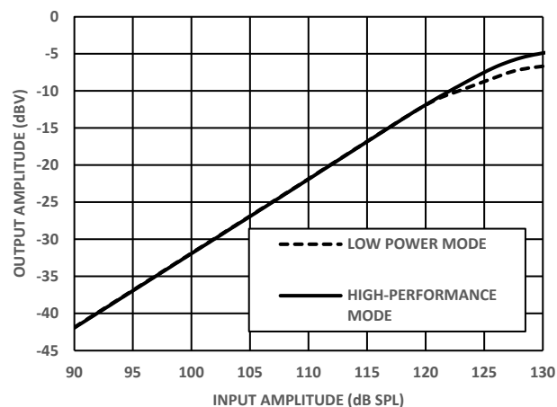
Figure 6. Linearity
