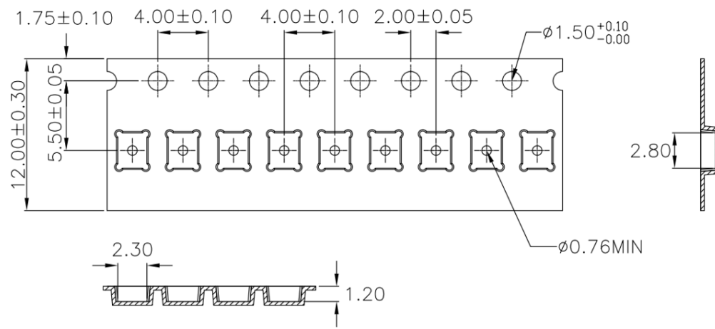
Figure 9. ICP-10111 Tape Dimensions
