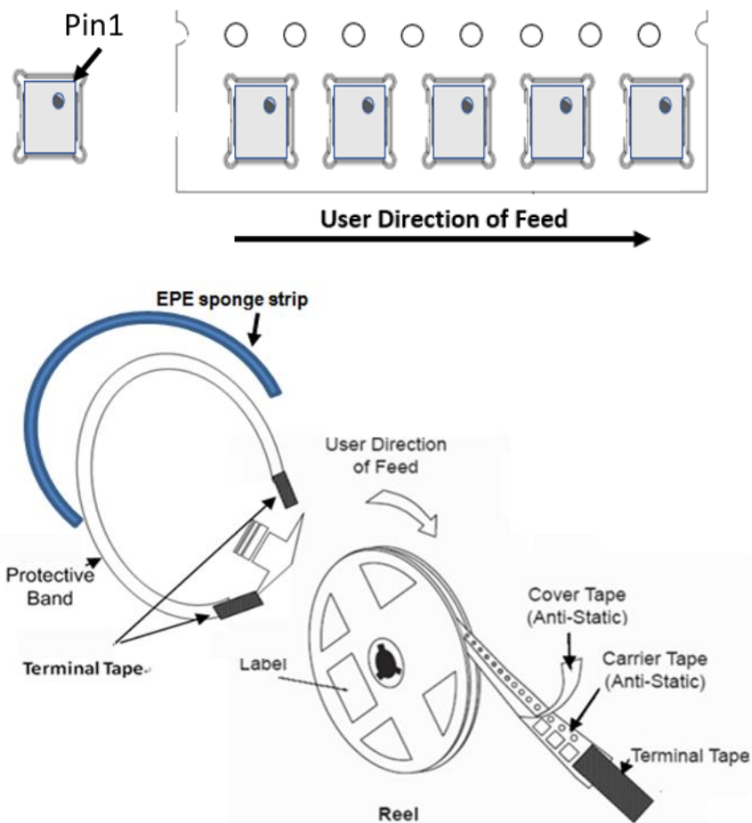
Figure 10. ICP-10111 Tape and Reel Drawing
