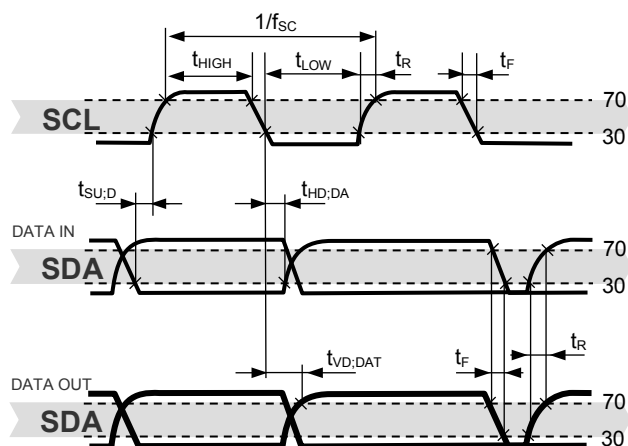
Figure 1. Digital I/O Pads Timing
