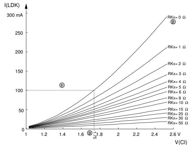
Figure 9: Diode current vs. V(CI) at Tj = 27 °C
