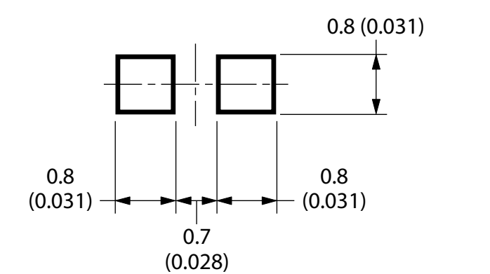
Figure 13: Recommended Soldering Pattern for HSMx-C190, C191, and C197
