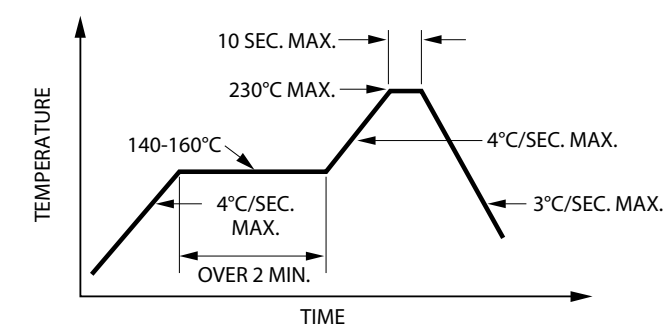
Figure 9: Recommended Reflow Soldering Profile
