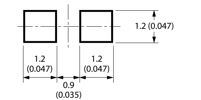
Figure 12: Recommended Soldering Pattern for HSMx-C170 and C177
