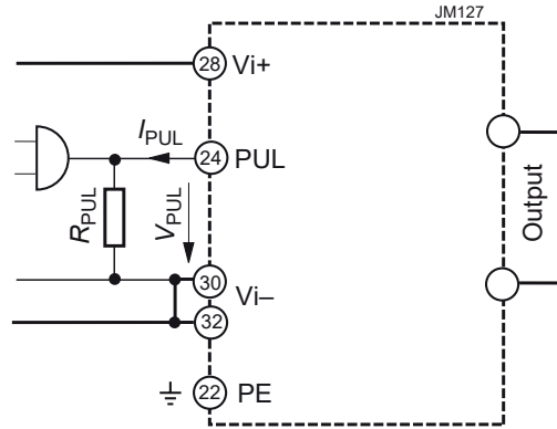
Fig. 16 Circuit for the inhibit function
