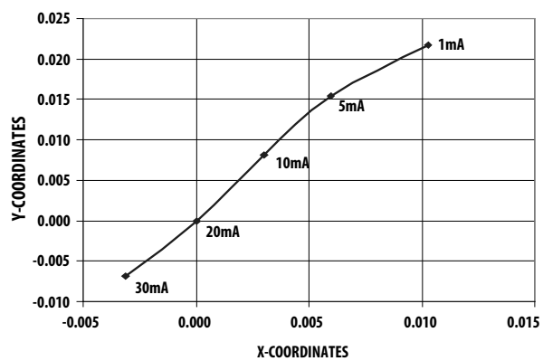
Figure 4. Chromaticity shift vs Forward Current
