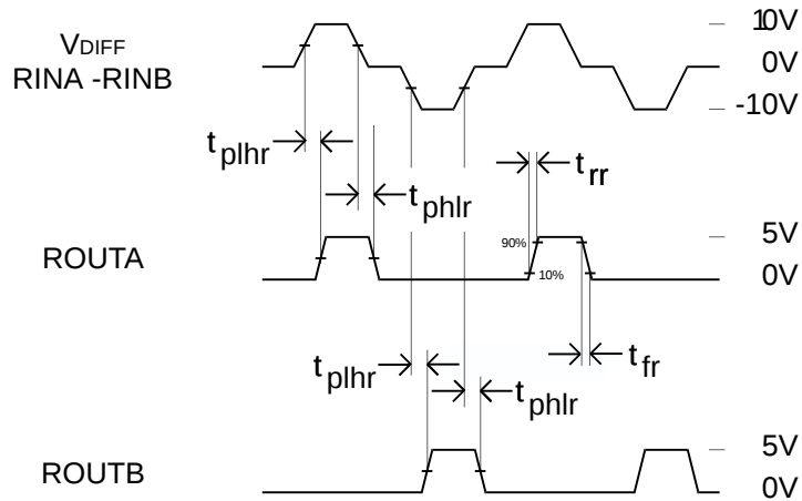
FIGURE 5 - RECEIVER TIMING
