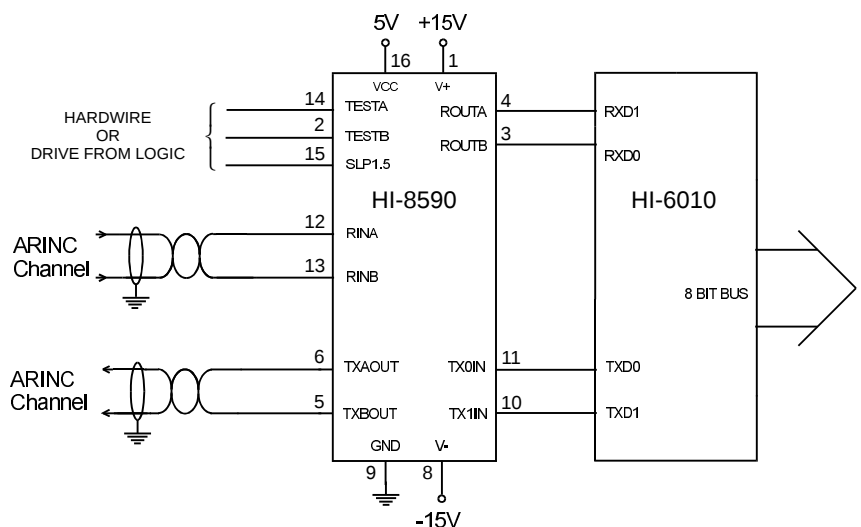
FIGURE 3 - APPLICATION DIAGRAM
