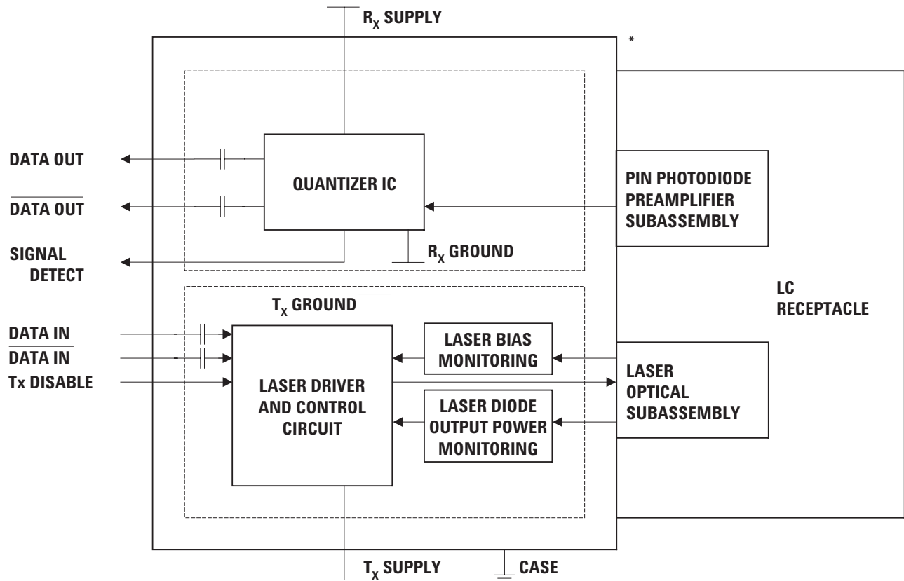
Figure 3. Block Diagram
