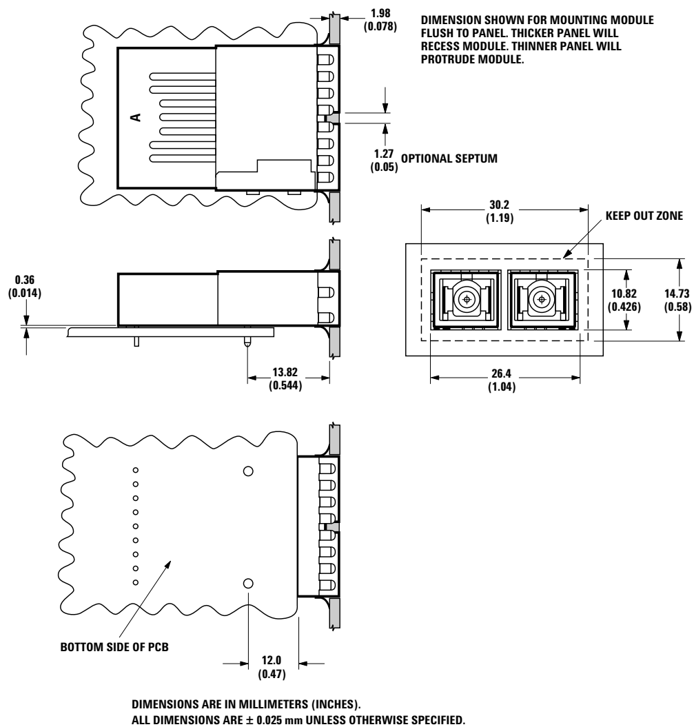
Figure 9. Suggested Module Positioning and Panel Cut-out for HFBR/HFCT-53D5FM.
