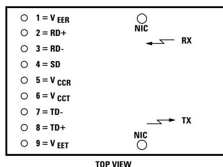
Figure 2. Pin-Out.
