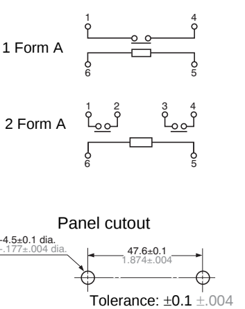
Schematic (Bottom view) Single side stable type
