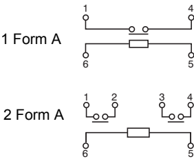
Schematic (Bottom view) Single side stable type
