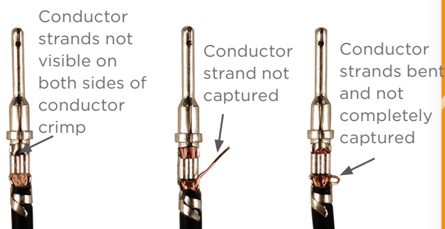
Unacceptable Crimps
