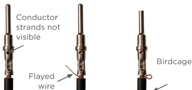
Unacceptable Crimps
