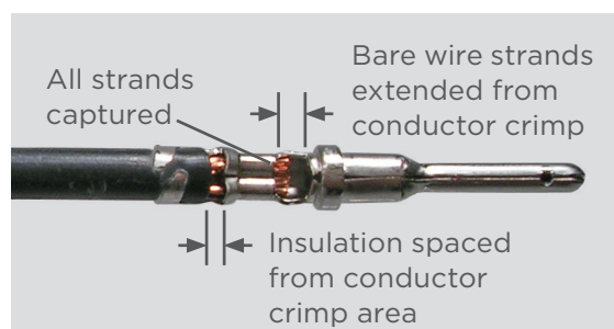
Acceptable Crimp
