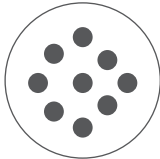
HD10-9-96P-N005 9 size 16
