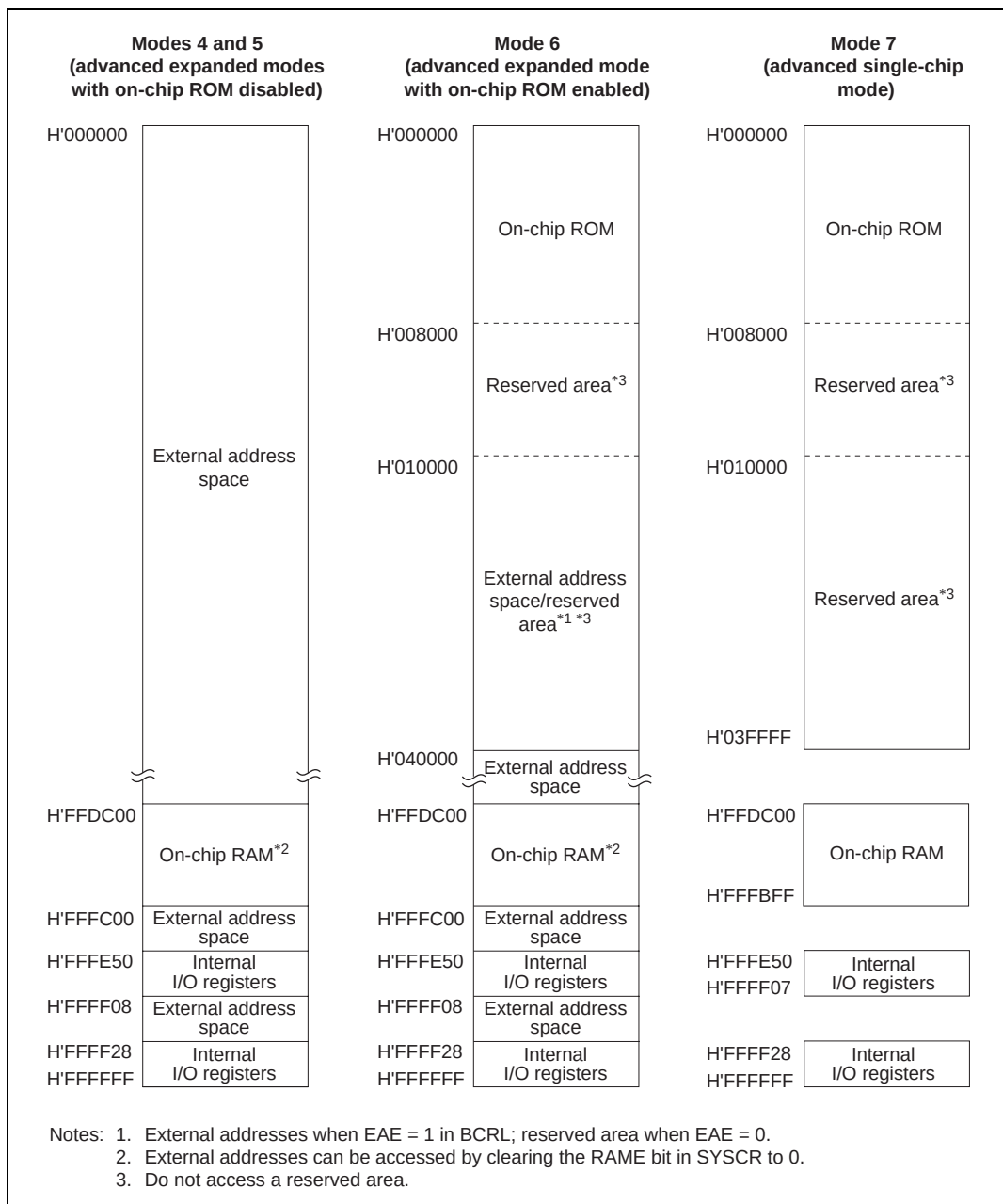
Figure 3.6 H8S/2323 Memory Map in Each Operating Mode
