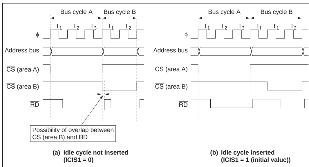
Figure 6.33 Relationship between Chip Select ( \overline{\text{CS}} ) and Read ( \overline{\text{RD}} )
