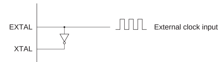
Figure 20.6 External Clock Input Timing
