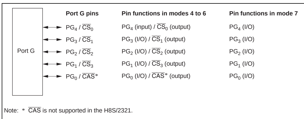
Figure 9.23 Port G Pin Functions
