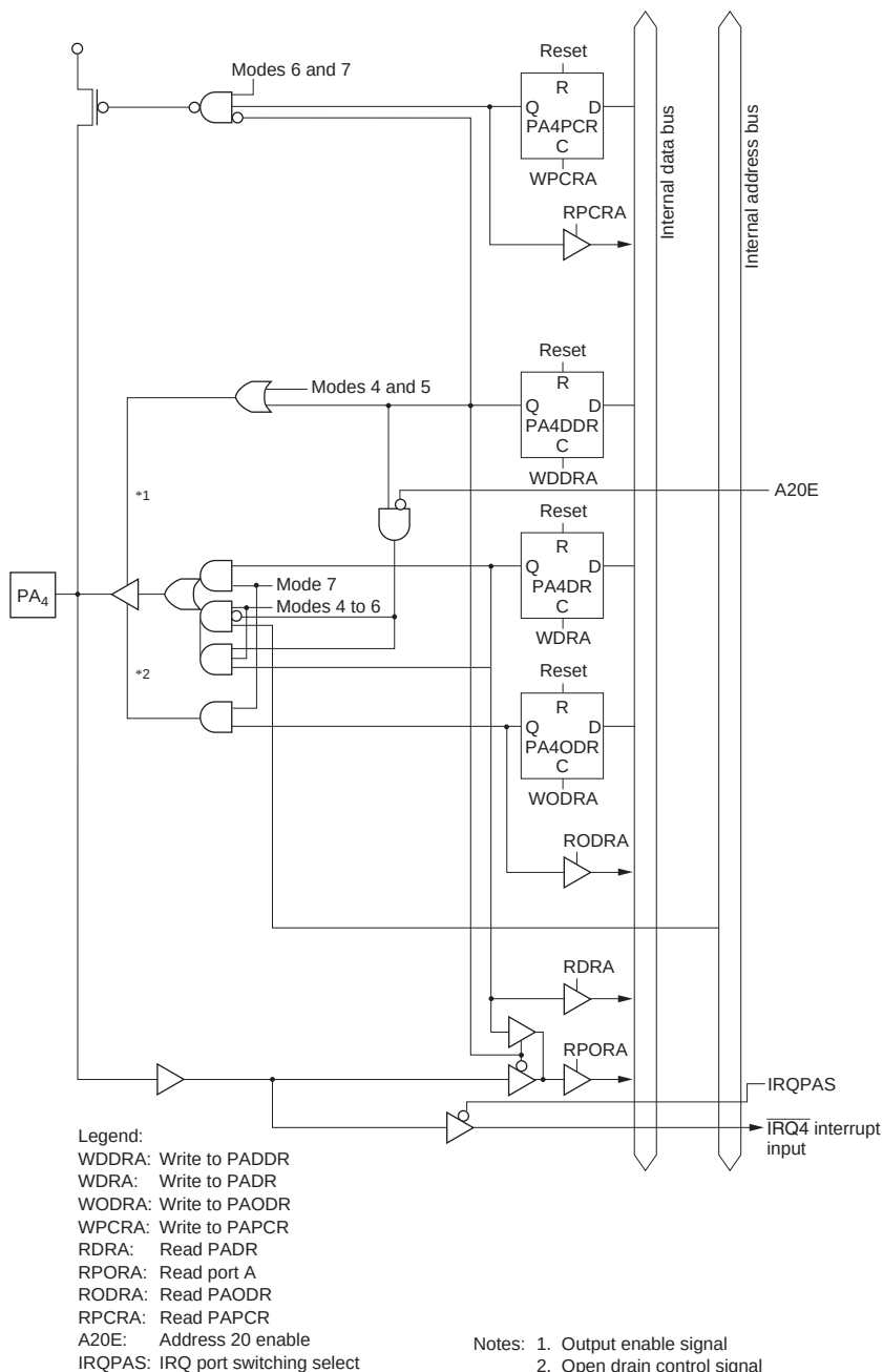
Figure C.7 (b) Port A Block Diagram (Pin PA 4 )
