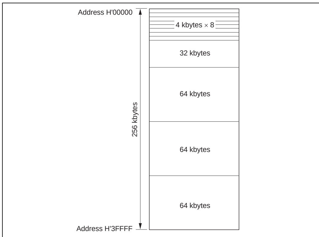
Figure 19.35 Flash Memory Block Configuration
