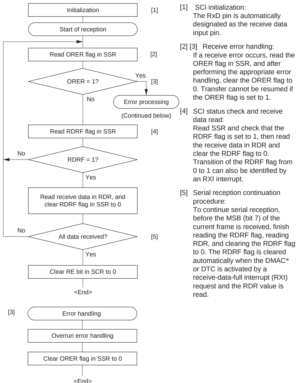
Figure 14.18 Sample Serial Reception Flowchart
