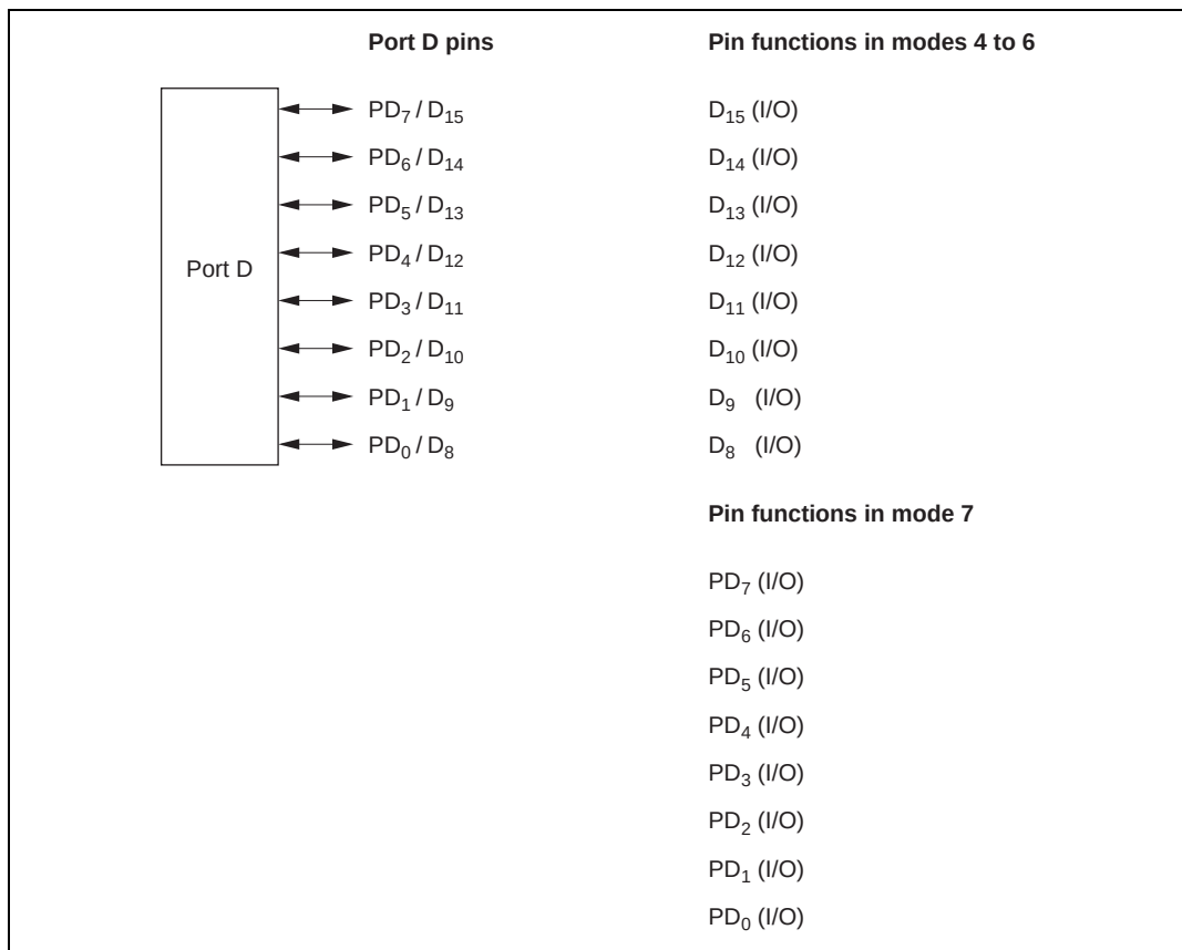
Figure 9.16 Port D Pin Functions
