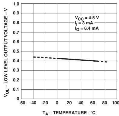
Figure 6. Typical Logic Low Output Voltage vs. Temperature.
