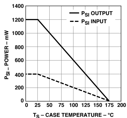
Figure 37b. HCPL-315J: Thermal Derating Curve, Dependence of Safety Limiting Value with Case Temperature per IEC/EN/DIN EN 60747-5-5.
