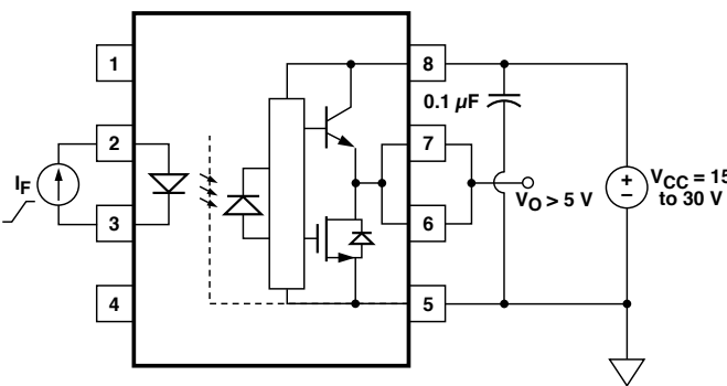
Figure 21. I_{FH} Test Circuit.
