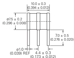
Radial Leaded with-FT (GTCR38-XXXM-R10-FT)
