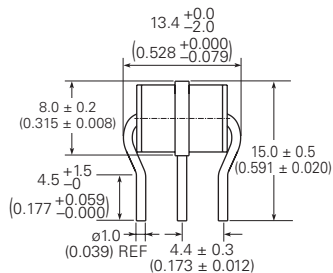
Axial Leaded with-FT (GTCA38-XXXM-R10-FT)
