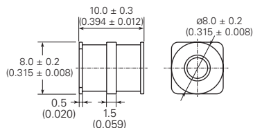
Surface-mount (GTCS38-XXXM-R10)
