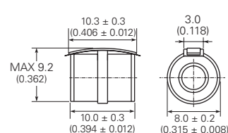
No Leads with-FT (GTCN38-XXXM-R10-FT)†
