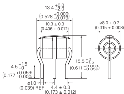
Radial Leaded (GTCR38-XXXM-R10)
