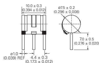
Radial Leaded with-FS (GTCR38-XXXM-R10-FS2)
