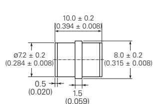
No Leads (GTCN38-XXXM-R10)†
