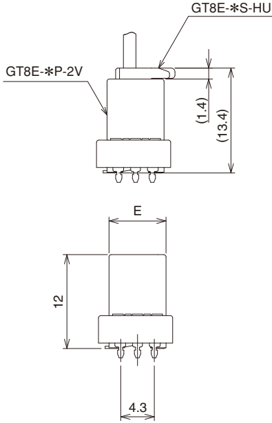
◆Fitting diagram
