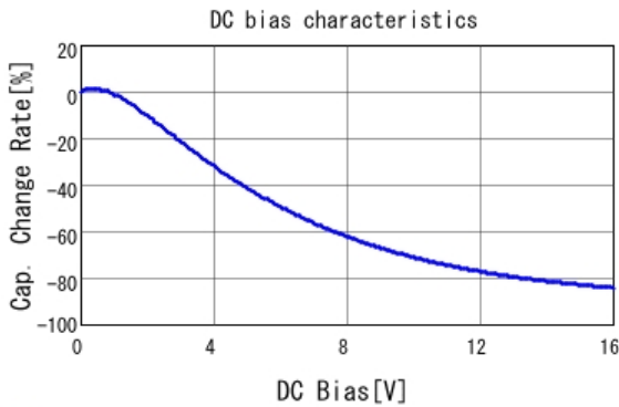
■ GRT32EC81C476KE13 C-DC bias capchange, 25.0degC, AC0.
