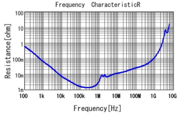
■ GRT32EC81C476KE13 R DCOV, 25degC
