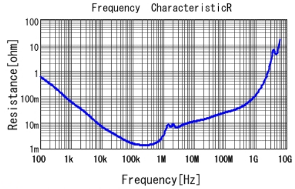
■ GRT32EC81A476KE13 R DCOV, 25degC
