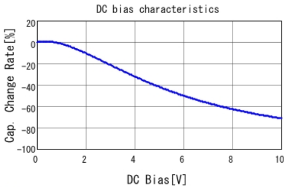
■ GRT32EC81A476KE13 C-DC bias capchange, 25.0degC, AC0.
