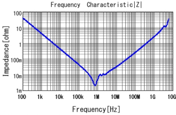
■ GRT32EC81A476KE13 |Z| DCOV, 25degC
