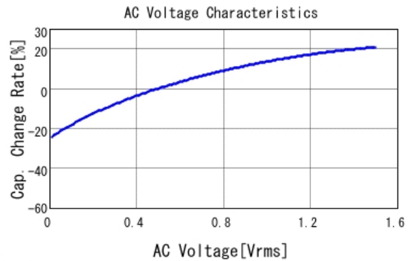
■ GRT32EC81A476KE13 C-AC Voltage capchange, DCOV, 25.0d
