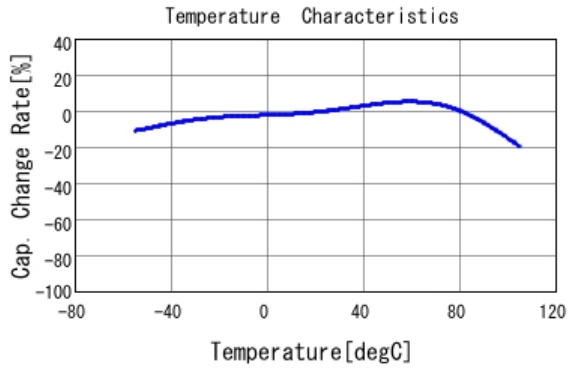
■ GRT32EC81A476KE13 C-Temp. capchange, DC0.0V, AC0.5Vrm
