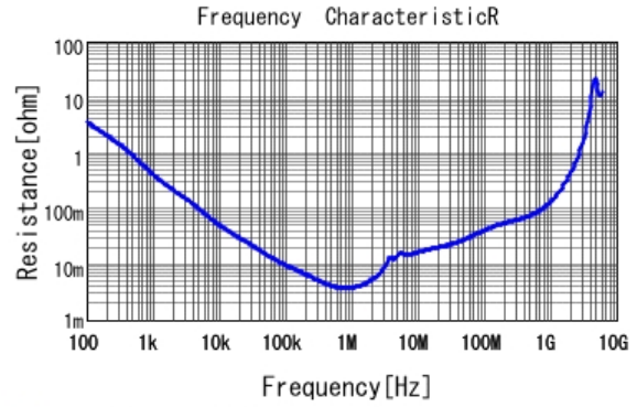
■ GRT31CR61H106KE01 R DCOV, 25degC
