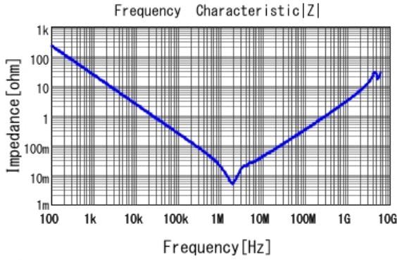
■ GRT31CR61H106KE01 |Z| DCOV, 25degC
