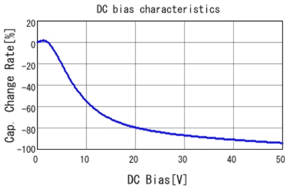
■ GRT31CR61H106KE01 C-DC bias capchange, 25.0degC, AC1.
