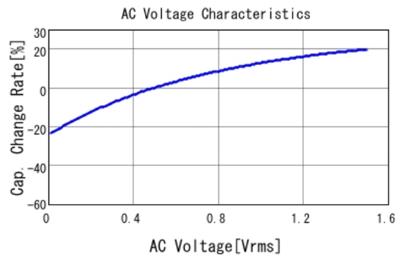
■ GRT31CR61E226KE01 C-AC Voltage capchange, DCOV, 25.0d
