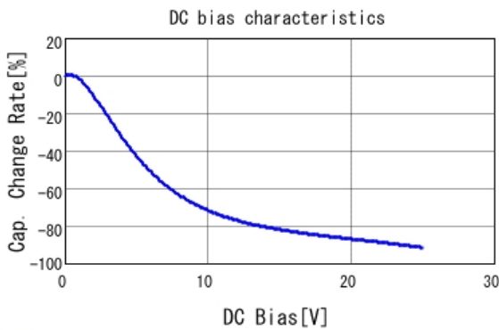
■ GRT31CR61E226KE01 C-DC bias capchange, 25.0degC, AC0.
