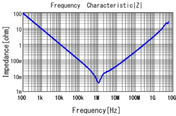
■ GRT31CR61E226KE01 |Z| DCOV, 25degC
