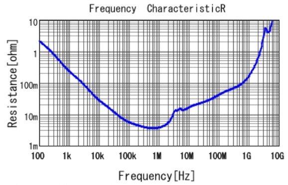
■ GRT31CR61E106ME01 R DCOV, 25degC
