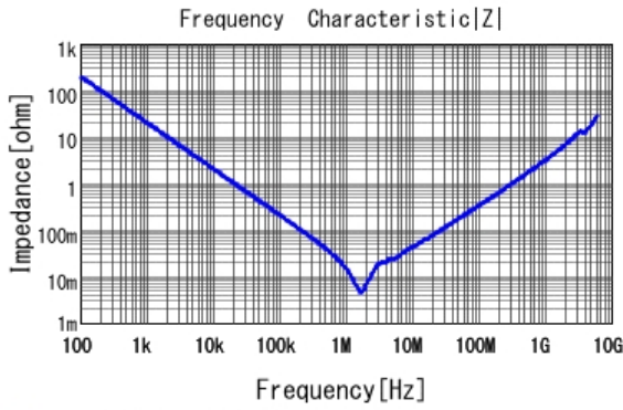
■ GRT31CR61E106KE01 |Z| DC0V, 25degC
