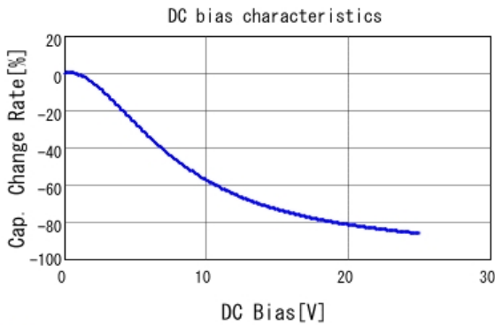
■ GRT31CR61E106KE01 C-DC bias capchange, 25.0degC, AC1.
