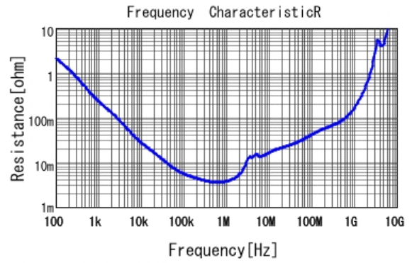
■ GRT31CR61E106KE01 R DC0V, 25degC
