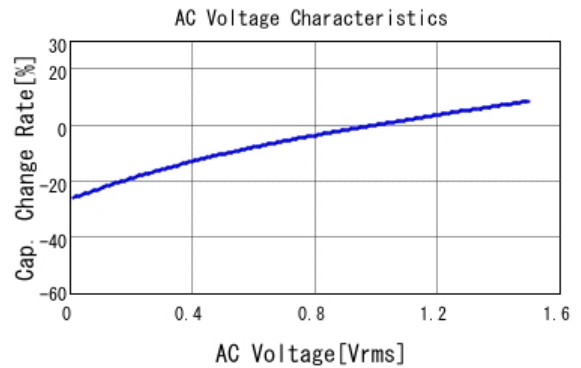
■ GRT31CR61E106KE01 C-AC Voltage capchange, DC0V, 25.0d
