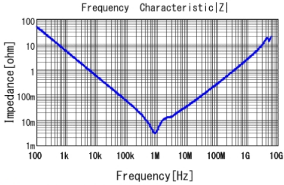
■ GRT31CR61A476KE13 |Z| DCOV, 25degC
