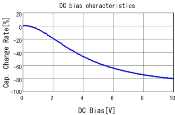
■ GRT31CR61A476KE13 C-DC bias capchange, 25.0degC, AC0.
