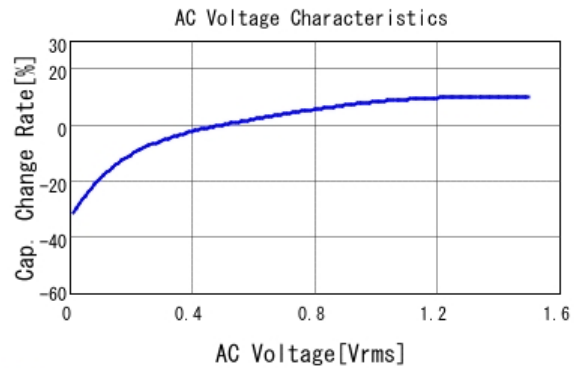
■ GRT31CR61A476KE13 C-AC Voltage capchange, DCOV, 25.0d
