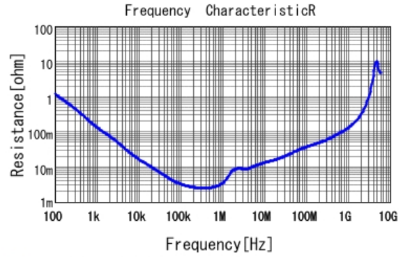
■ GRT31CR61A476KE13 R DCOV, 25degC
