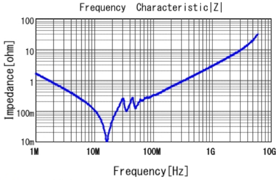
■ GRT31C5C1E104JA02 |Z| DC0V, 25degC
