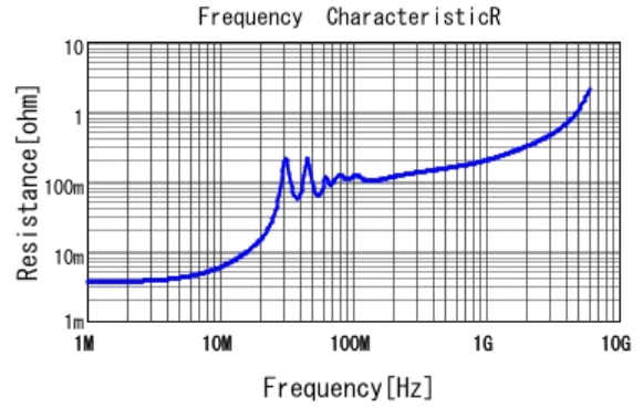
■ GRT31C5C1E104JA02 R DC0V, 25degC
