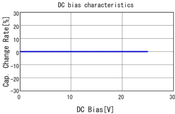
■ GRT31C5C1E104JA02 C-DC bias capchange, 25.0degC, AC1V
