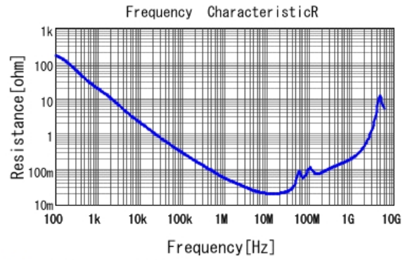
■ GRT21BR72A473KE01 R DCOV, 25degC
