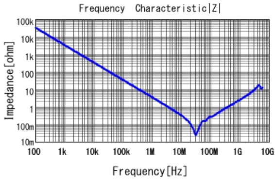
■ GRT21BR72A473KE01 |Z| DCOV, 25degC
