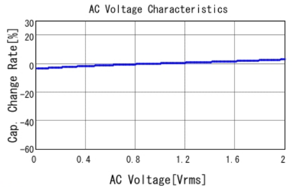
■ GRT21BR72A473KE01 C-AC Voltage capchange, DCOV, 25.0d
