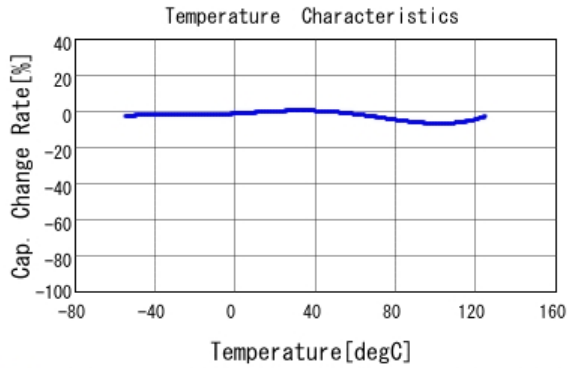
■ GRT21BR72A473KE01 C-Temp. capchange, DC0.0V, AC1.0Vrm
