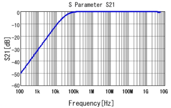
■ GRT21BR72A473KE01 S21 DC0V, 25degC
