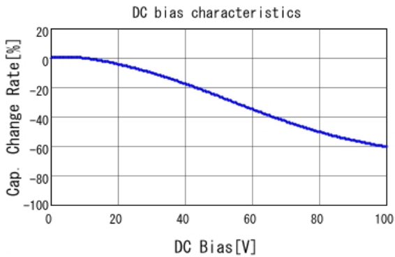
■ GRT21BR72A473KE01 C-DC bias capchange, 25.0degC, AC1.
