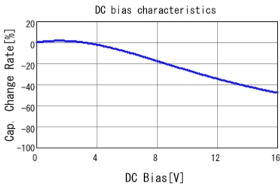
■ GRT21BR71C225KE01 C-DC bias capchange, 25.0degC, AC1.
