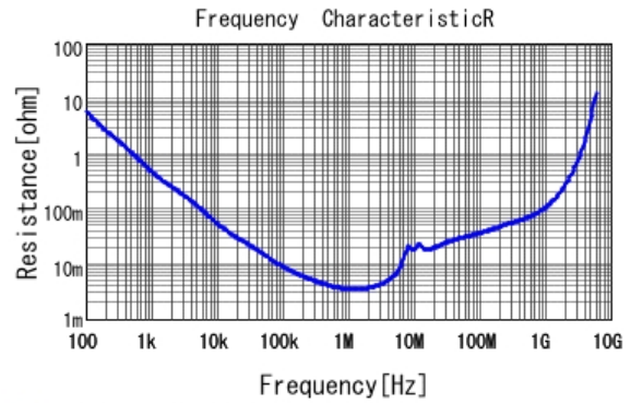
■ GRT21BR71C225KE01 R DC0V, 25degC
