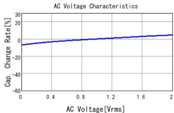
■ GRT21BR71C225KE01 C-AC Voltage capchange, DC0V, 25.0d
