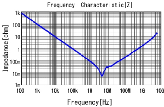
■ GRT21BR71C225KE01 |Z| DC0V, 25degC
