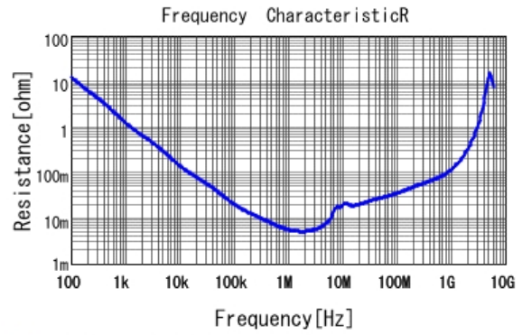
■ GRT21BR71A475KE13 R DCOV, 25degC
