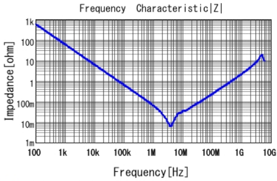
■ GRT21BR71A475KE13 |Z| DCOV, 25degC
