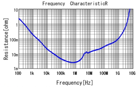
■ GRT21BR61C106KE01 R DC0V, 25degC
