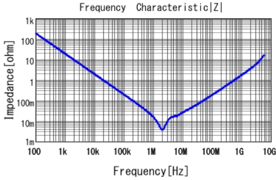
■ GRT21BR61C106KE01 |Z| DC0V, 25degC
