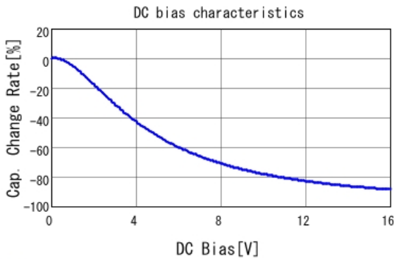
■ GRT21BR61C106KE01 C-DC bias capchange, 25.0degC, AC0.
