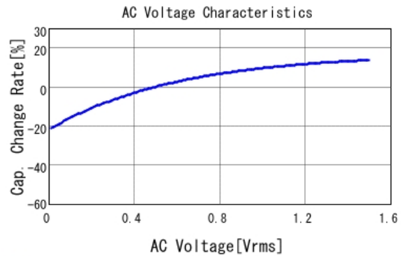
■ GRT21BR61A106KE01 C-AC Voltage capchange, DC0V, 25.0d
