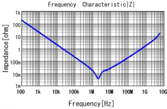
■ GRT21BR61A106KE01 |Z| DC0V, 25degC
