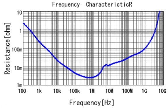
■ GRT21BR61A106KE01 R DC0V, 25degC
