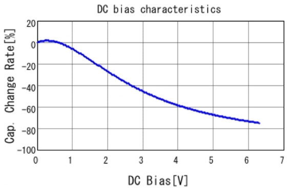
■ GRT21BR60J476ME13 C-DC bias capchange, 25.0degC, AC0.
