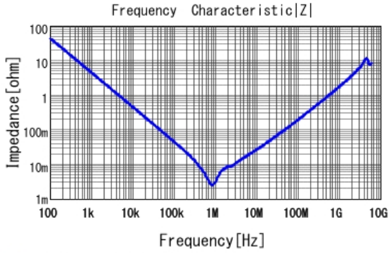
■ GRT21BR60J476ME13 |Z| DCOV, 25degC
