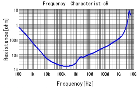
■ GRT21BR60J476ME13 R DCOV, 25degC
