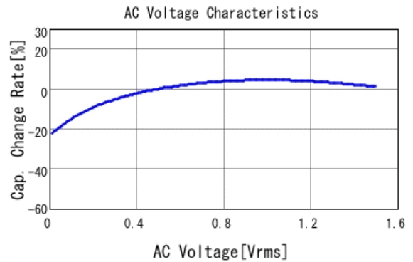
■ GRT21BR60J476ME13 C-AC Voltage capchange, DCOV, 25.0d
