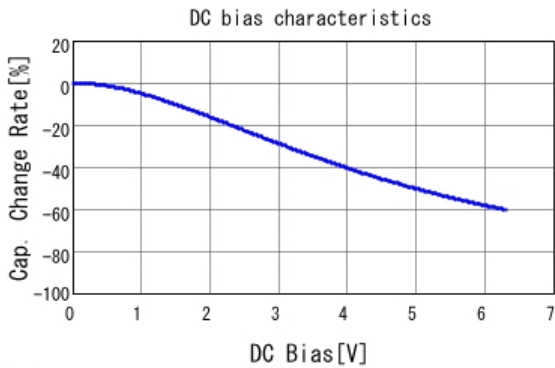
■ GRT21BR60J106KE01 C-DC bias capchange, 25.0degC, AC0.
