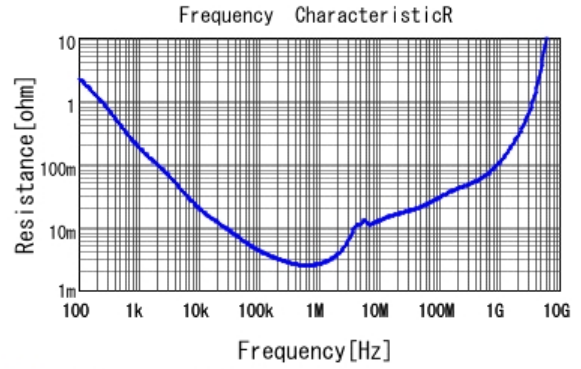
■ GRT21BR60J106KE01 R DCOV, 25degC
