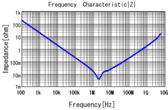
■ GRT21BR60J106KE01 |Z| DCOV, 25degC
