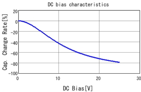
■ GRT21BC81E335KE13 C-DC bias capchange, 25.0degC, AC1.
