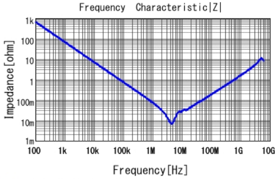
■ GRT21BC81E335KE13 |Z| DCOV, 25degC
