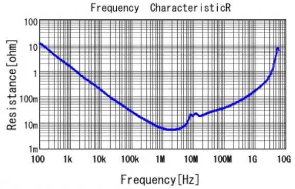
■ GRT21BC81E335KE13 R DCOV, 25degC
