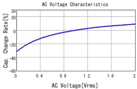
■ GRT21BC81E335KE13 C-AC Voltage capchange, DCOV, 25.0d
