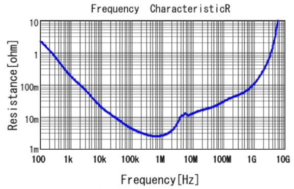
■ GRT21BC81C106KE01 R DCOV, 25degC
