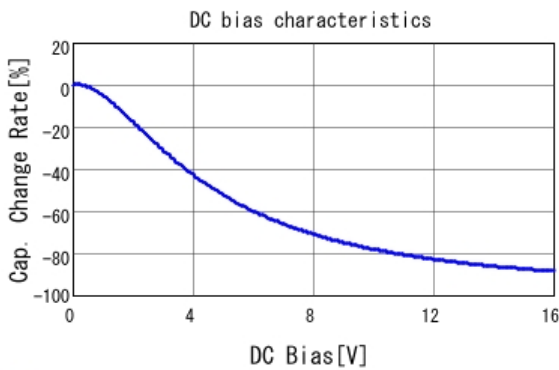
■ GRT21BC81C106KE01 C-DC bias capchange, 25.0degC, AC0.
