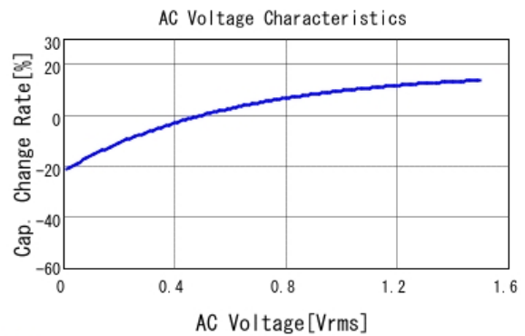
■ GRT21BC81C106KE01 C-AC Voltage capchange, DCOV, 25.0d
