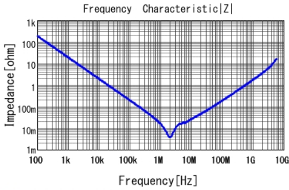
■ GRT21BC81C106KE01 |Z| DCOV, 25degC
