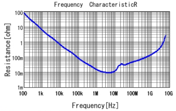
■ GRT188R71E105KE13 R DCOV, 25degC
