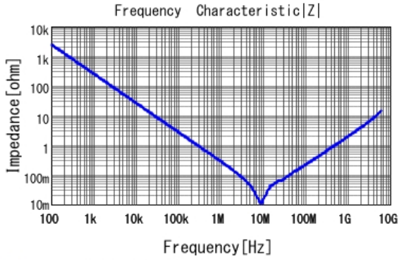
■ GRT188R71E105KE13 |Z| DCOV, 25degC
