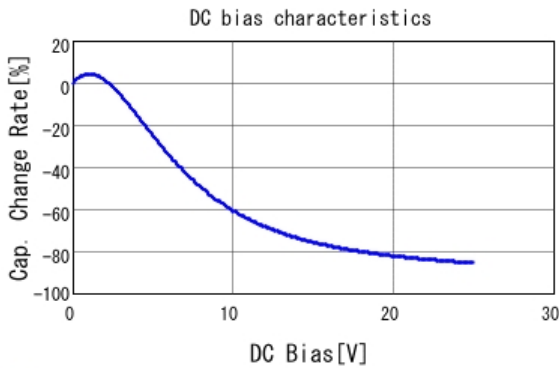
■ GRT188R71E105KE13 C-DC bias capchange, 25.0degC, AC1.
