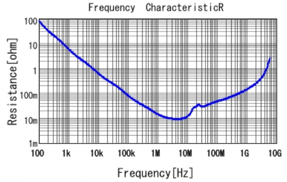
■ GRT188R71C105KE13 R DCOV, 25degC
