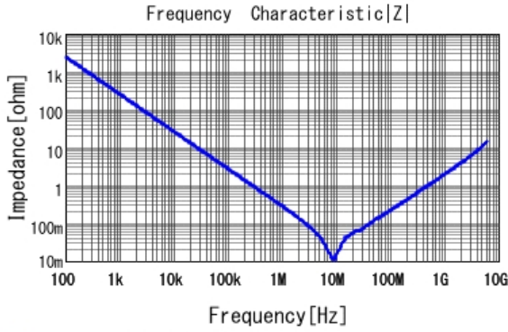
■ GRT188R71C105KE13 |Z| DCOV, 25degC
