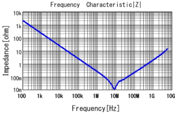
■ GRT188R6YA105KE13 |Z| DCOV, 25degC
