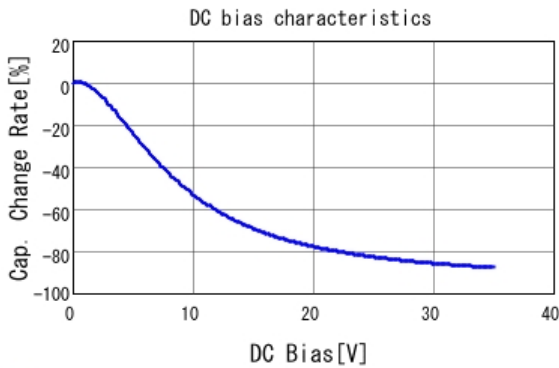
■ GRT188R6YA105KE13 C-DC bias capchange, 25.0degC, AC1.
