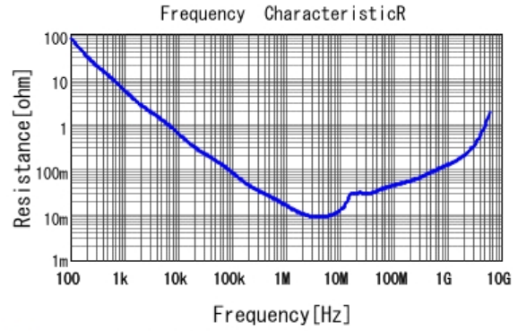
■ GRT188R6YA105KE13 R DCOV, 25degC
