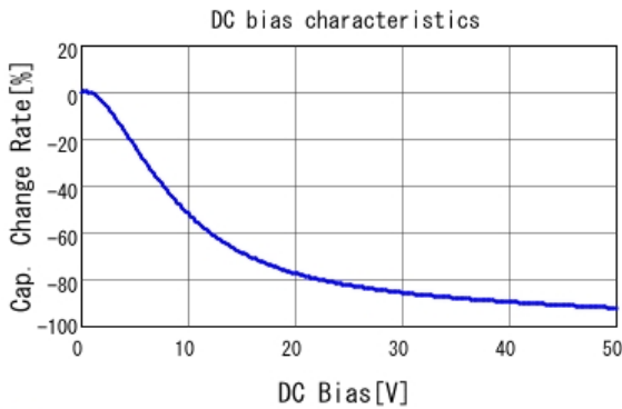
■ GRT188R61H105KE13 C-DC bias capchange, 25.0degC, AC1.
