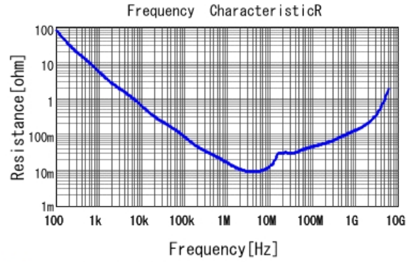
■ GRT188R61H105KE13 R DCOV, 25degC
