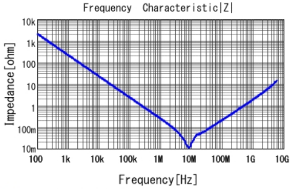
■ GRT188R61H105KE13 |Z| DCOV, 25degC
