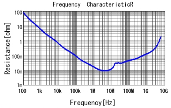
■ GRT188R61C105KE13 R DCOV, 25degC
