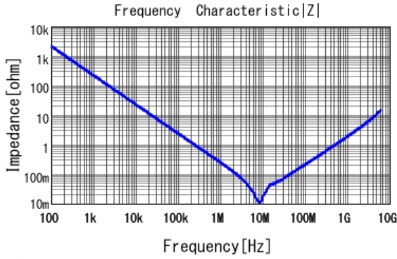
■ GRT188R61C105KE13 |Z| DCOV, 25degC
