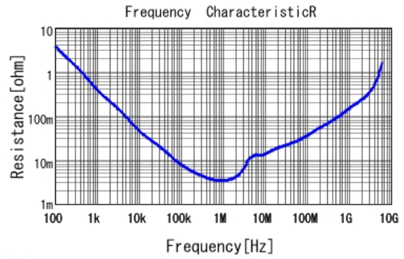
■ GRT188D71A106ME13 R DCOV, 25degC
