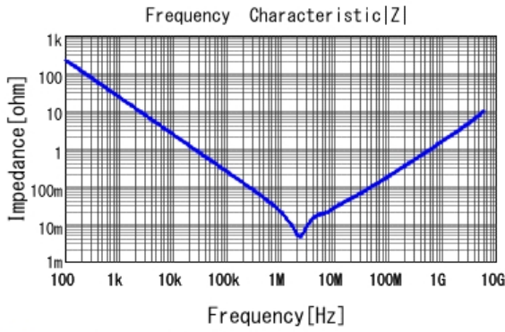
■ GRT188D71A106ME13 |Z| DCOV, 25degC
