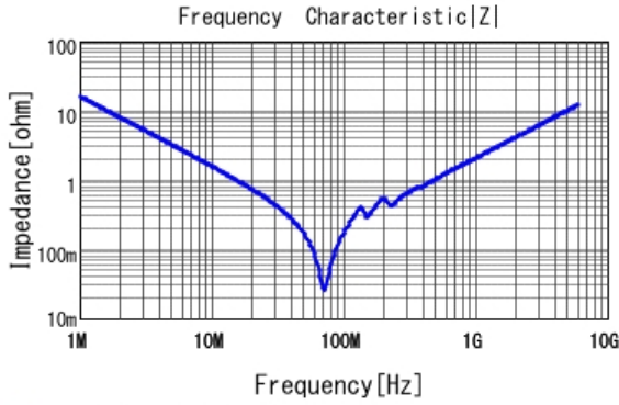
■ GRT1885C1H103JA02 |Z| DCOV, 25degC
