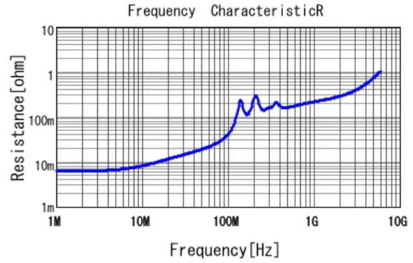
■ GRT1885C1H103JA02 R DCOV, 25degC
