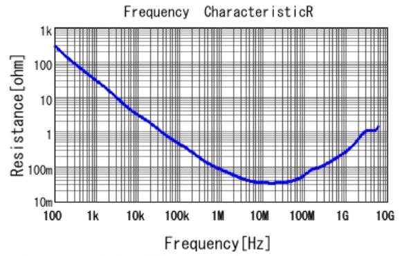
■ GRT155R71H333KE01 R DC0V, 25degC
