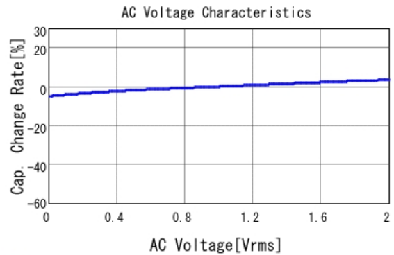
■ GRT155R71H333KE01 C-AC Voltage capchange, DC0V, 25.0d
