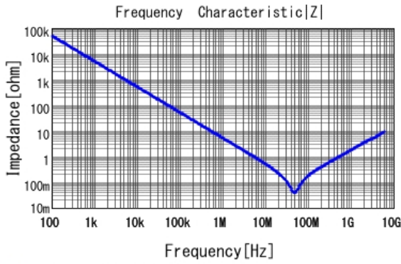
■ GRT155R71H333KE01 |Z| DC0V, 25degC
