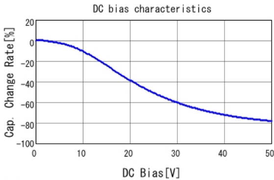
■ GRT155R71H333KE01 C-DC bias capchange, 25.0degC, AC1.
