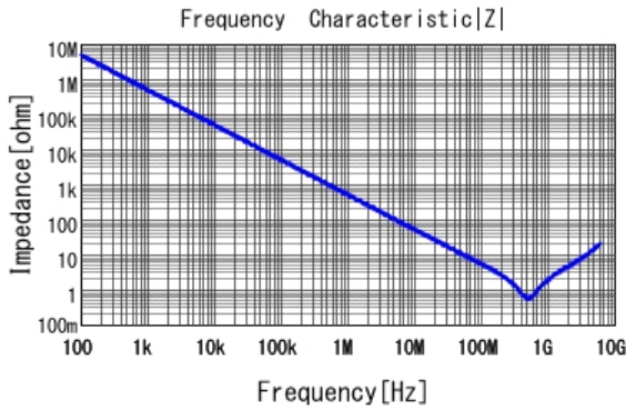
■ GRT155R71H331KE01 |Z| DCOV, 25degC
