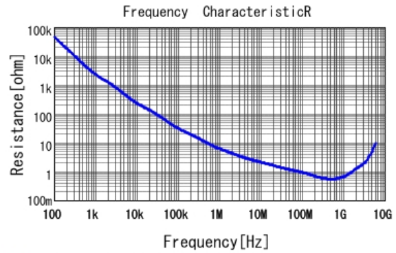
■ GRT155R71H331KE01 R DCOV, 25degC
