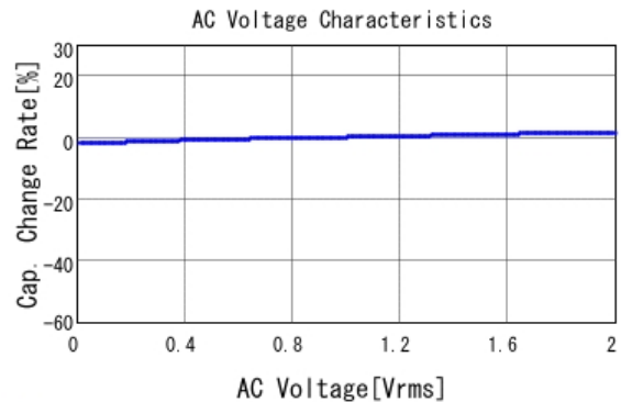
■ GRT155R71H331KE01 C-AC Voltage capchange, DCOV, 25.0d
