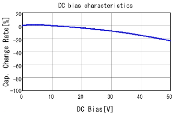
■ GRT155R71H331KE01 C-DC bias capchange, 25.0degC, AC1.
